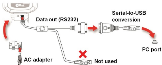
Connect via mini-USB/DB9 cable and DB9-to-USB adapter and use AC adapter for power
